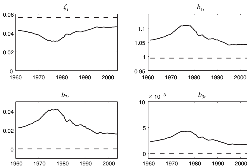
FIGURE 4. NKPC COEFFICIENTS
